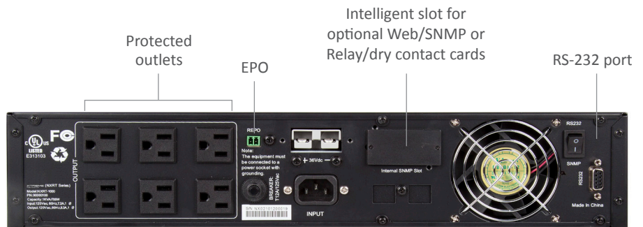
NXRT-1000 rear view
